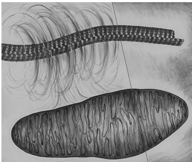
Fig. 1: Schematic drawing of energy excitation of a microtubule by a mitochondrion.
